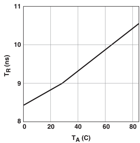
Figure 5: Typical Rise Time vs. Temperature
