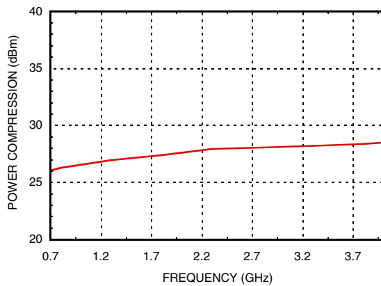
P0.1dB Vs. Frequency @ VDD= 3V, T_A = +25^\circ \text{C}
