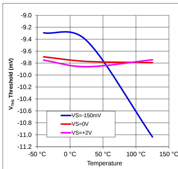
Figure 20: V_{TH1} vs. Temperature and Common Mode (OVT=Floating)
