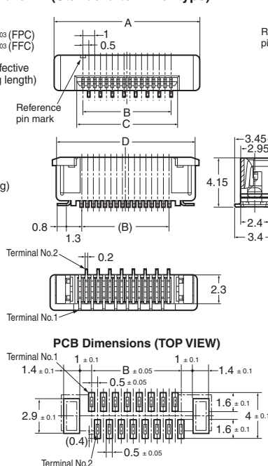
(Standard terminal type)
