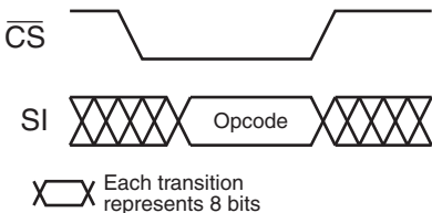
Figure 10-1. Deep Power-down
