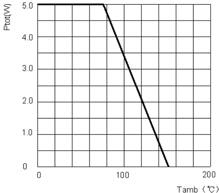
FIG1: Admissible Power Dissipation vs. Ambient Temperat
