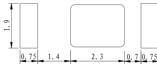
Recommended Soldering Pad
