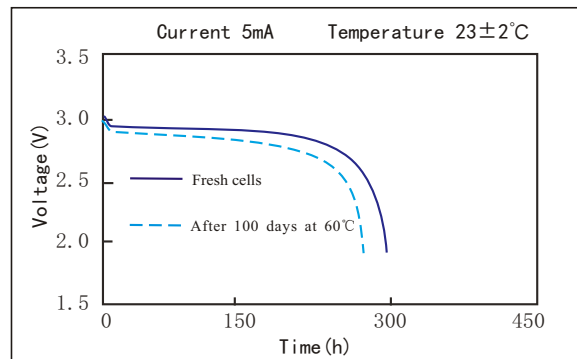
Storage characteristics
