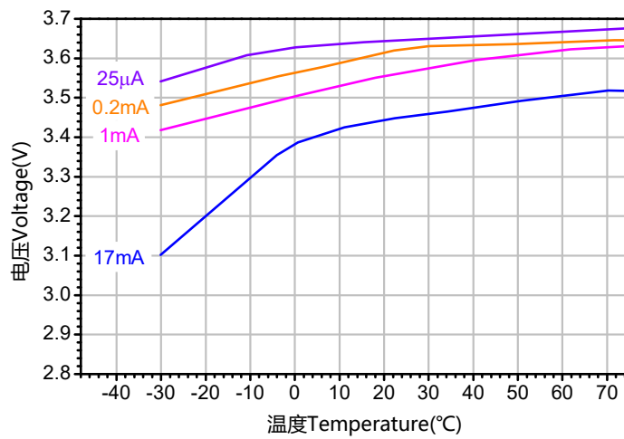
Voltage Versus Temperature
