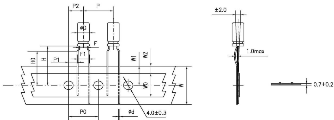
DIMENSIONS(mm)
