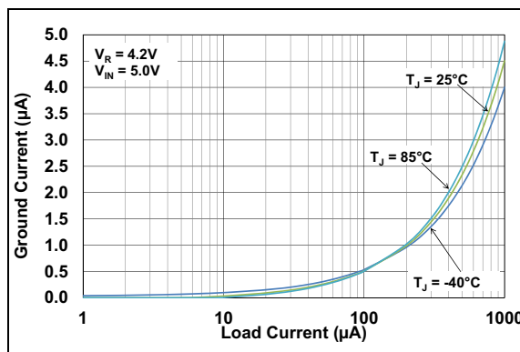
FIGURE 2-59: Ground Current vs. Very Low Load Current ( V_R = 4.2V ).
