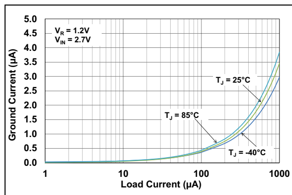
FIGURE 2-56: Ground Current vs. Very Low Load Current ( V_R = 1.2V ).
