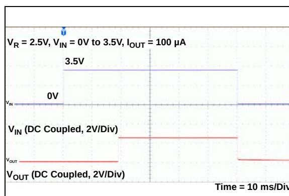
FIGURE 2-29: Start-up from V_{IN} ( V_R = 2.5\text{V} ).
