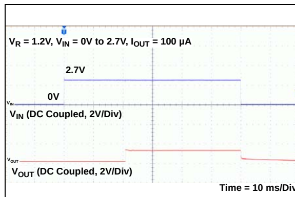
FIGURE 2-28: Start-up from V_{IN} ( V_R = 1.2\text{V} ).
