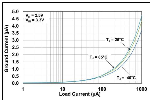
FIGURE 2-57: Ground Current vs. Very Low Load Current ( V_R = 2.5V ).
