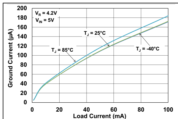
FIGURE 2-55: Ground Current vs. Load Current ( V_R = 4.2V ).
