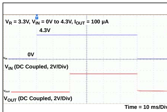
FIGURE 2-30: Start-up from V_{IN} ( V_R = 3.3\text{V} ).
