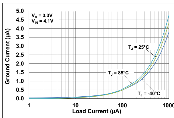
FIGURE 2-58: Ground Current vs. Very Low Load Current ( V_R = 3.3V ).
