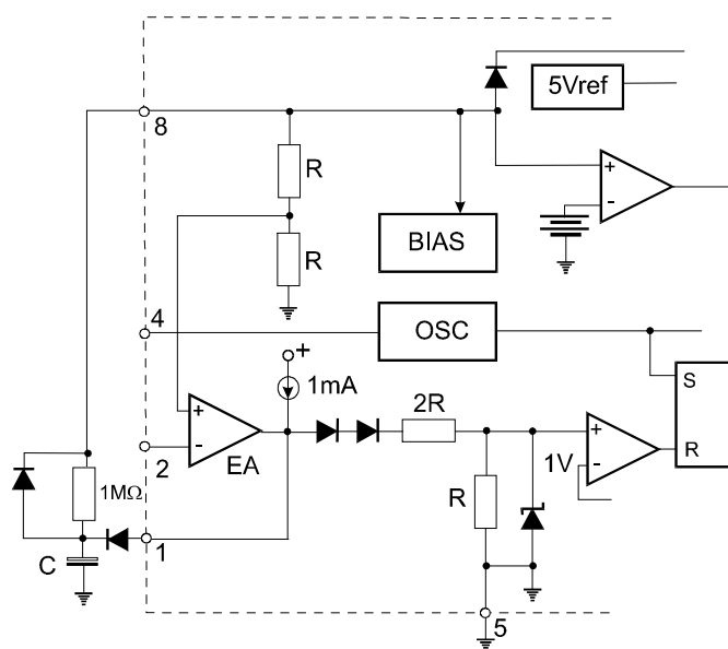
Figure 8. Soft-Start Circuit
