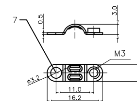
MIDDLE WASHER
