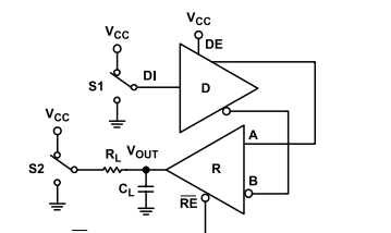
Figure 43. Receiver Enable/Disable from Shutdown
