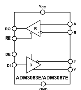
Figure 2. ADM3063E/ADM3067E Functional Block Diagram
