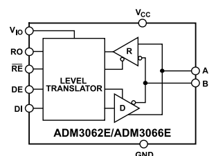
Figure 3. ADM3062E/ADM3066E Functional Block Diagram
