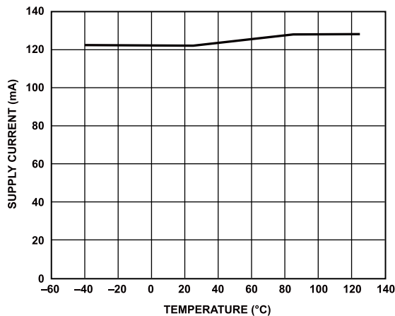
Figure 22. Supply Current ( I_{CC} ) vs. Temperature, Data Rate = 500 kbps, 500 kbps Models, V_{CC} = 5.5\text{ V}
