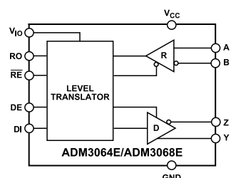
Figure 4. ADM3064E/ADM3068E Functional Block Diagram
