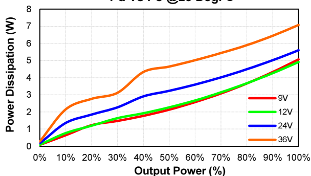
ECLB60W-24S15 Pd Vs Po @25 Deg. C
