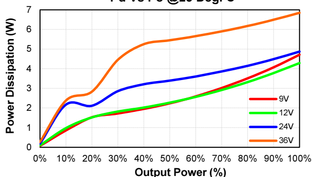
ECLB60W-24S12 Pd Vs Po @25 Deg. C
