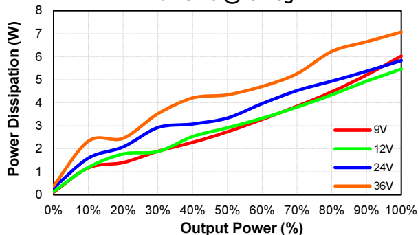
ECLB60W-24D12 Pd Vs Po @25 Deg. C
