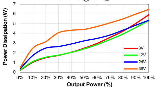
ECLB60W-24D15 Pd Vs Po @25 Deg. C
