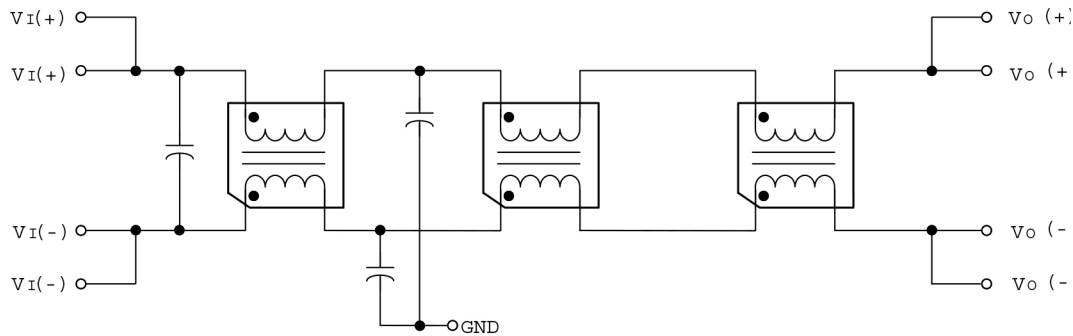
Figure 4. Internal Schematic
