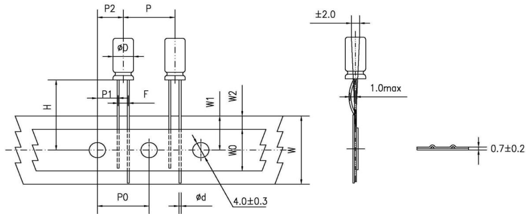
DIMENSIONS(mm)
