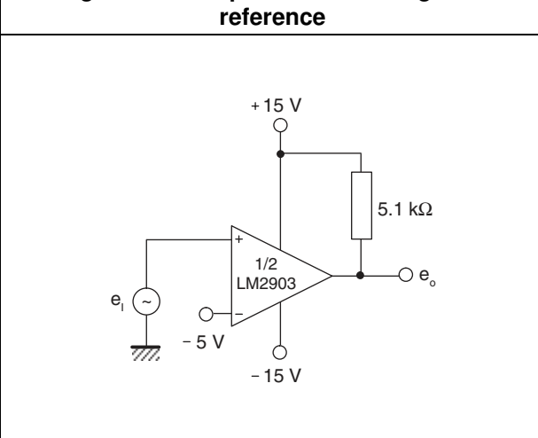
Figure 18. Comparator with a negative reference
