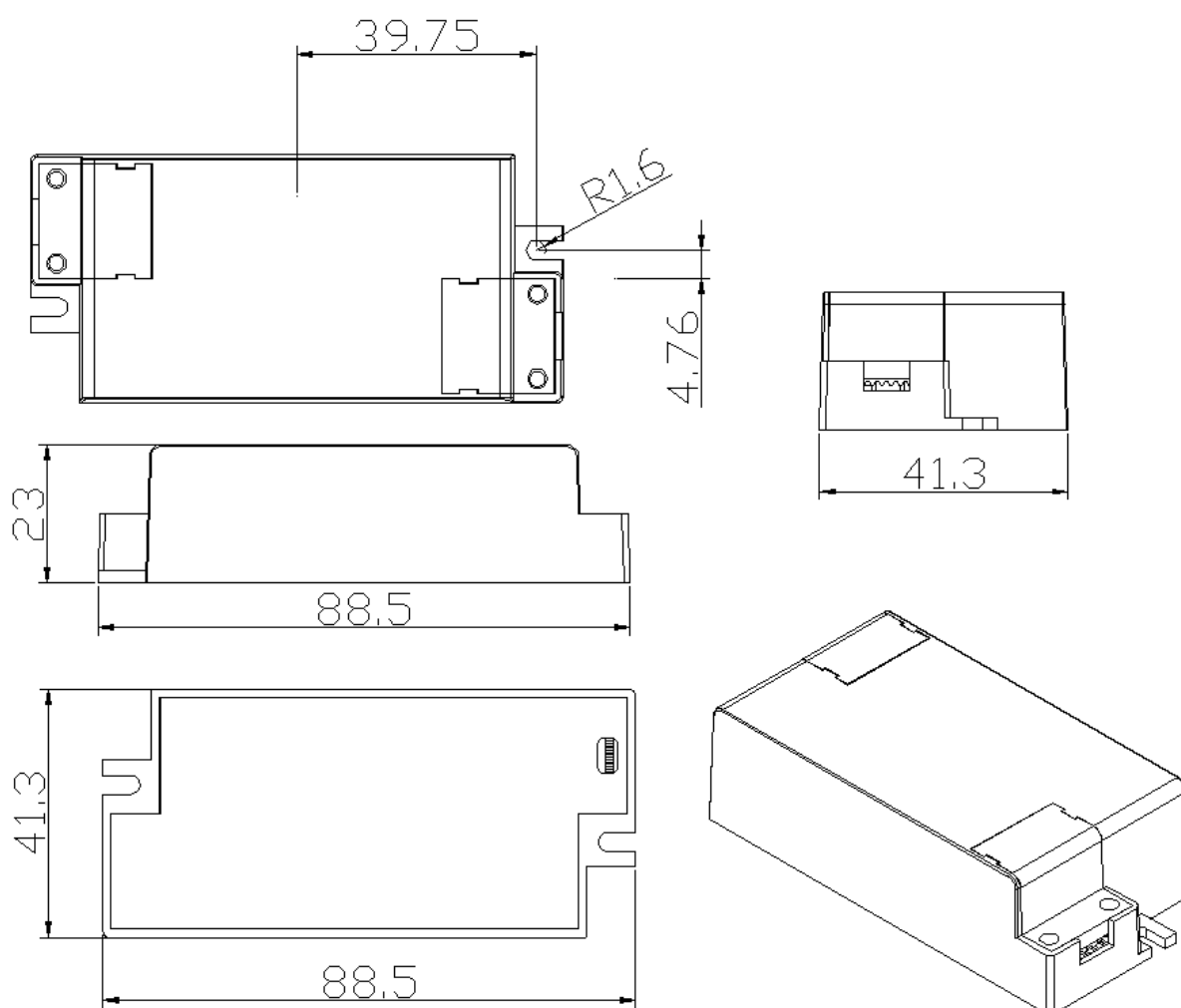
2D drawing :
