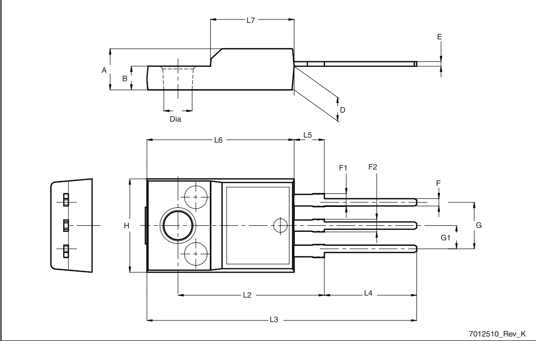
Figure 30. TO-220FP drawing
