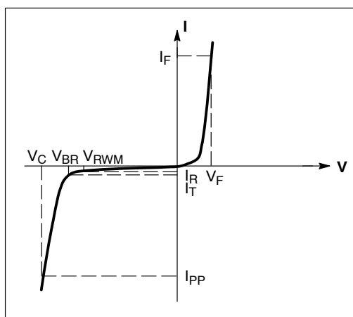
Uni-Directional
