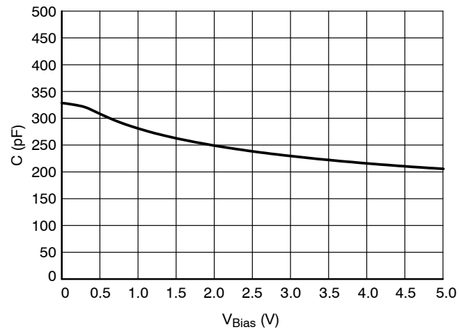
Figure 5. CV Characteristics
