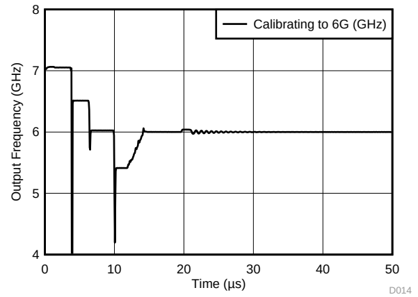
Figure 15. 20-μs Frequency Change Time to 6 GHz With Fast Calibration
