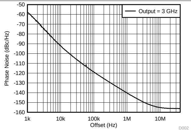
Figure 3. 3-GHz Output - Open-Loop Phase Noise
