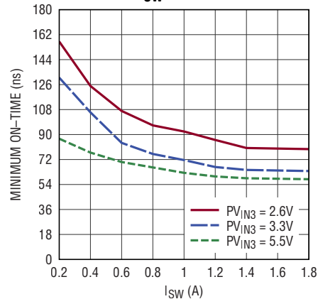
Channel 3 Minimum On-Time vs I_{SW}
