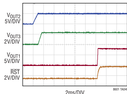
10V TO 24V TRANSIENTS TO 42V V_{IN} PV IN1 PV IN2 EN/UVLO TRKSS1 TRKSS2 RUN3 PG1 PG2 PG3 SYNC POREN RST CPOR RT GND LT8601 8601 TA04 OUT1 8V, 1.5A OUT2 5V, 1A OUT3 2.5V, 1.8A THE MAX CURRENT ON OUT2 IS I_{(OUT2)} = 2.5A - I_{PVIN3} - I_{BIAS}
