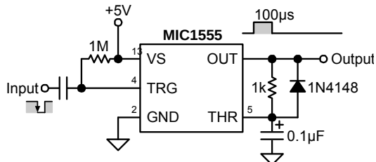
Figure 5. Falling-Edge Trigger Configuration
