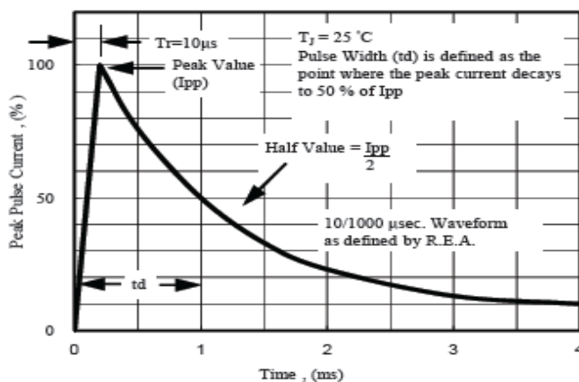
Fig. 5 - Pulse Waveform
