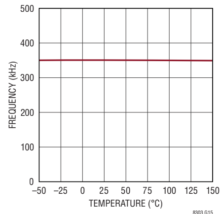
Maximum Switching Frequency
