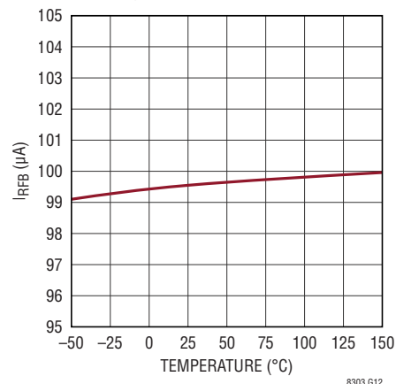
R_{\text{FB}} Regulation Current
