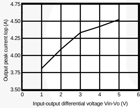
Figure 20. Output Peak Current vs. Input-Output Differential Voltage
