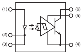
Internal circuit
