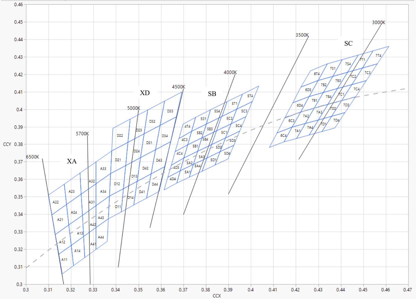
Bivariate Fit of CCY By CCX
