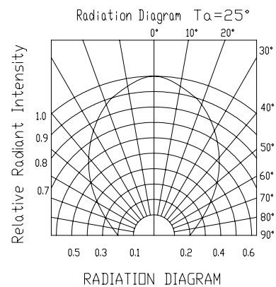
Relative Intensity vs. Angle Dispacemen
