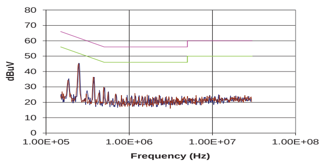
MEE1S1215XC
