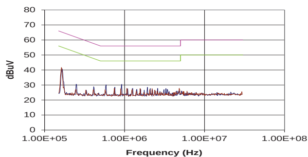
MEE1S2415XC
