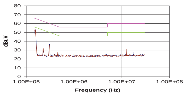
MEE1S1212XC
