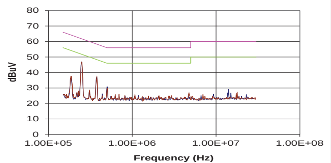
MEE1S0509XC
