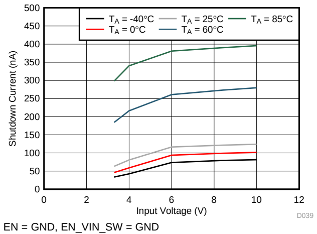
Figure 2. Shutdown Current
