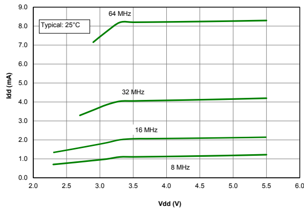
Figure 41-45. I_{DD} , ECH Oscillator, Typical, PIC18F65/66K40 only
