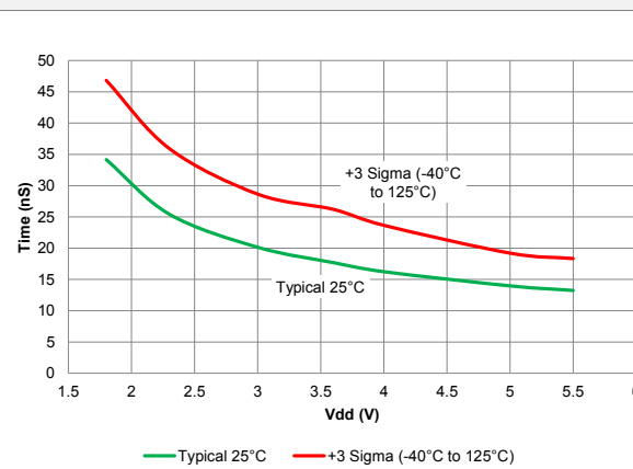
Figure 41-57. I/O Rise Time, Slew Rate Control Enabled
