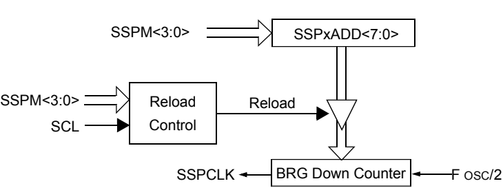
Figure 28-40. Baud Rate Generator Block Diagram
