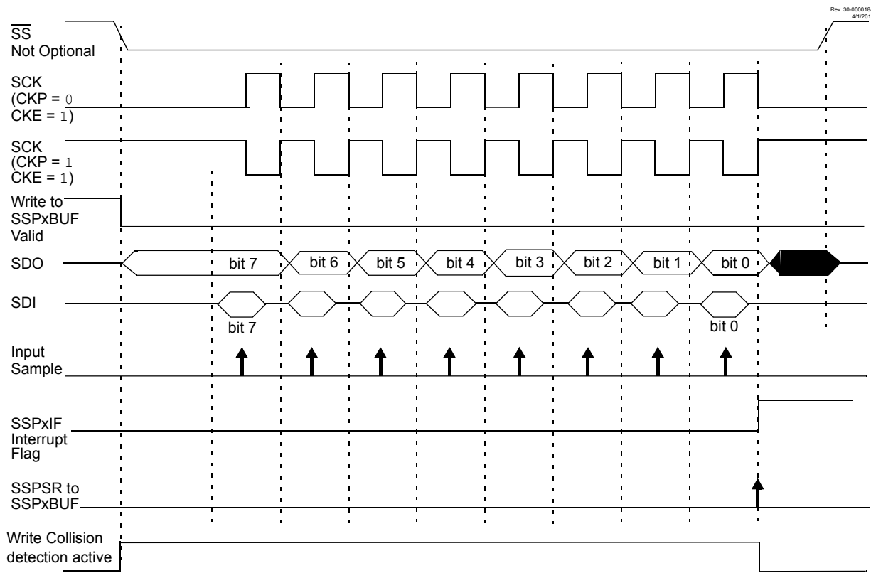
Figure 28-8. SPI Mode Waveform (Slave Mode with CKE = 1)
