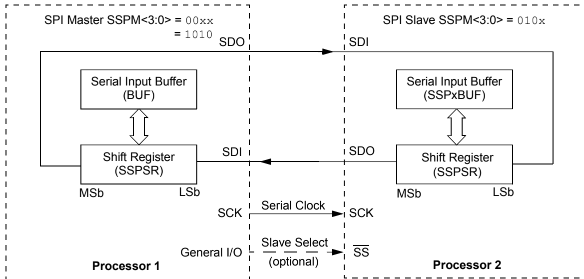
Figure 28-3. SPI Master/Slave Connection
