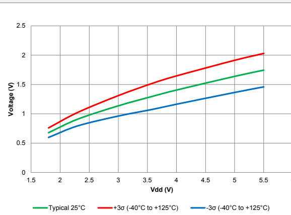
Figure 41-55. Schmitt Trigger Low Values
