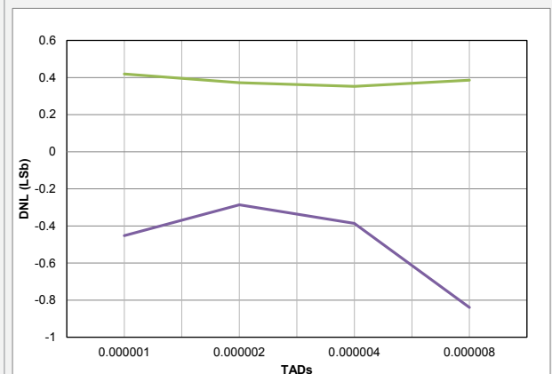
Figure 41-6. ADC, Single-Ended DNL, V_{DD} = 3.0V , V_{REF} = 3.0V
