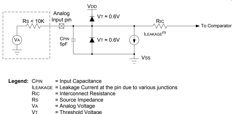
Figure 34-3. Analog Input Model
