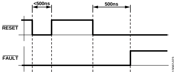
Figure 23. RESET Timing
