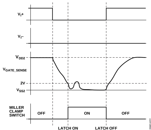
Figure 22. Miller Clamp Example
