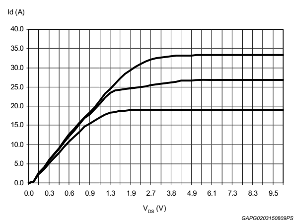
Figure 23. Output characteristics
