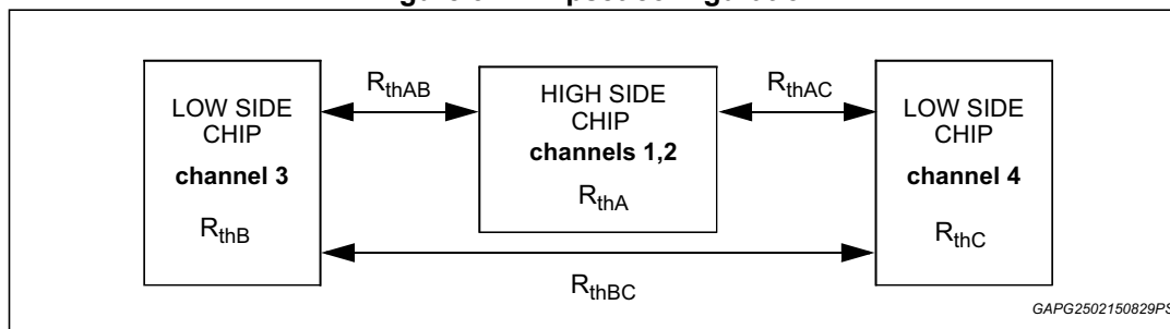
Figure 31. Chipset configuration
