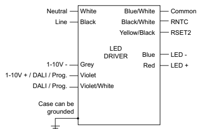
Xitanium 75W 0.70A Prog+ sXt
