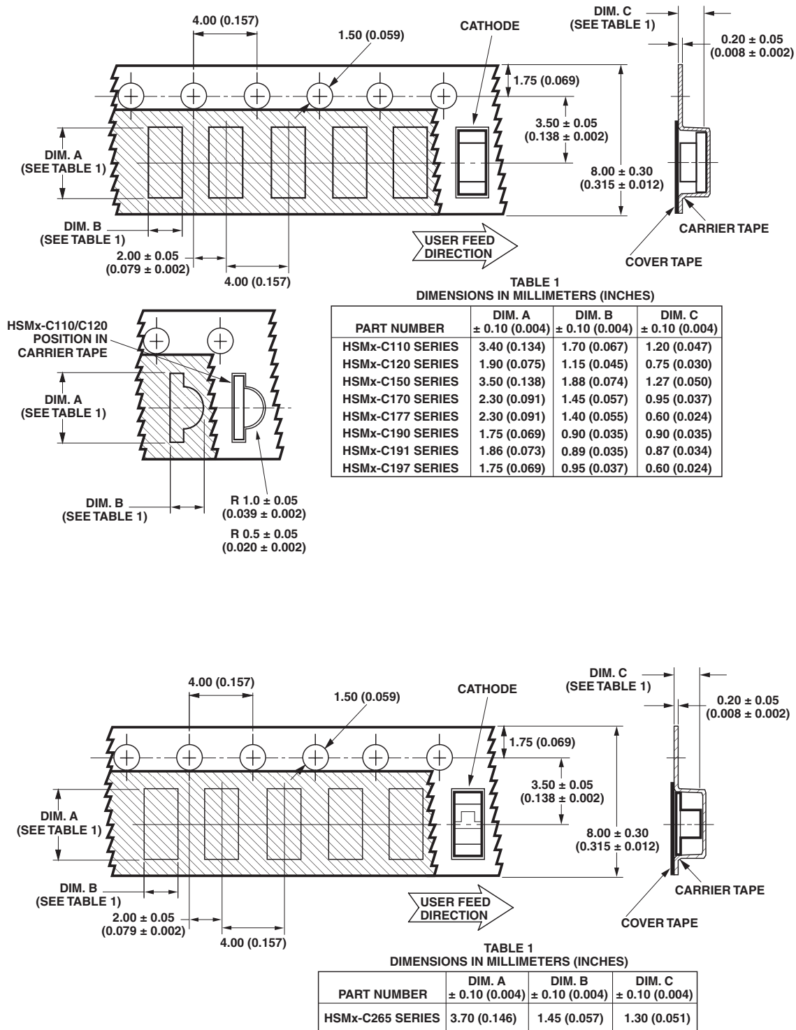
Figure 19. Tape dimensions.
