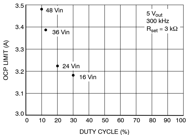
Figure 16. OCP Limit vs. Duty Cycle
