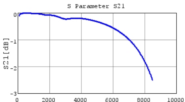
GRM1885C1H101JA01 S21 DCOV, 25degC
