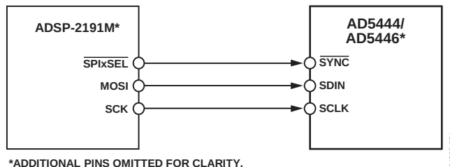
Figure 45. ADSP-2191M SPI to AD5444/AD5446 Interface
