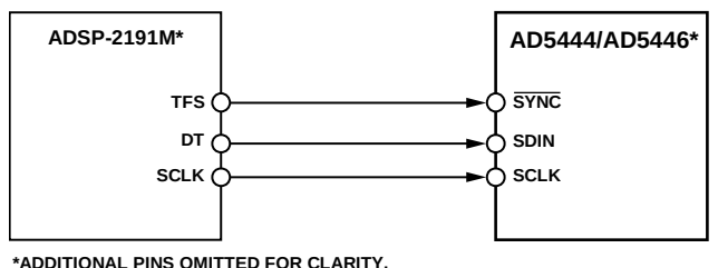
Figure 46. ADSP-2191M to AD5444/AD5446 Interface
