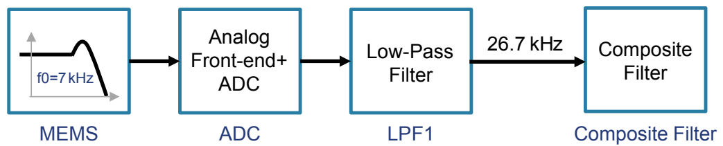
Figure 5. Filtering chain
