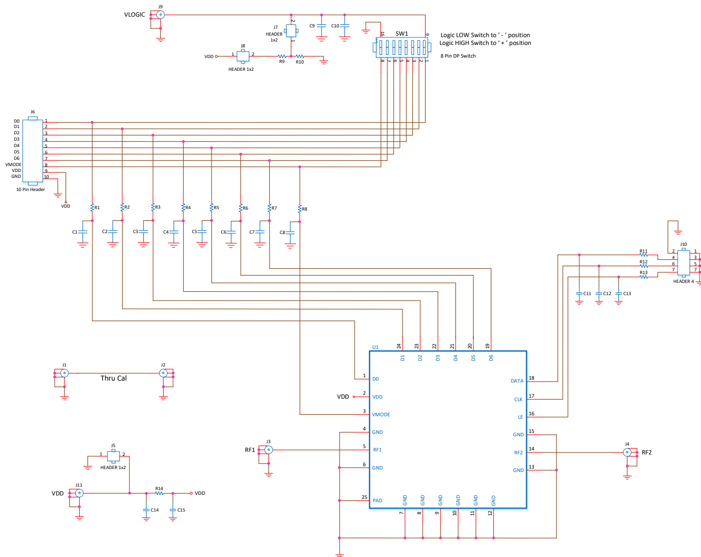
Figure 37. Electrical Schematic
