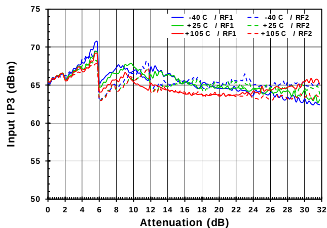
Figure 29. Input IP3 vs Attenuation [2GHz]
