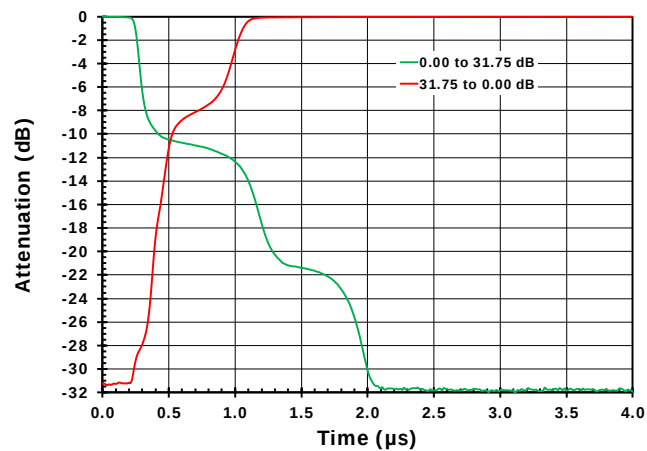
Figure 32. Switching Time between Maximum and Minimum Attenuation
