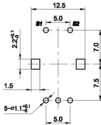
P.C.B. mounting hole detail
