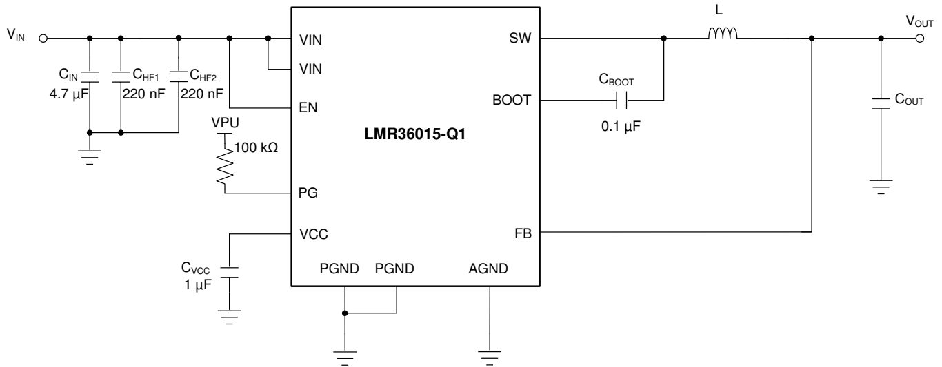
Figure 19. Example Applications Circuit (Fixed 3.3 V Output)
