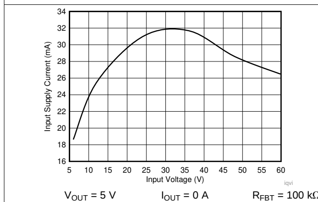
Figure 50. Input Supply Current
