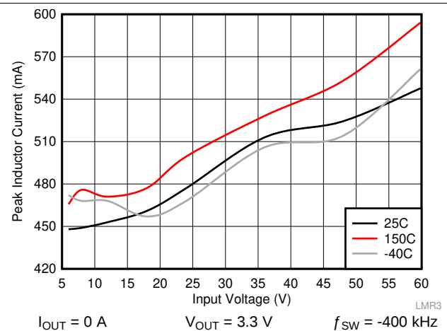
Figure 6. I_{PEAK-MIN}
