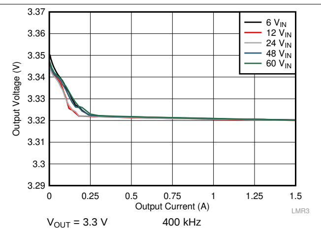
Figure 25. Load Regulation
