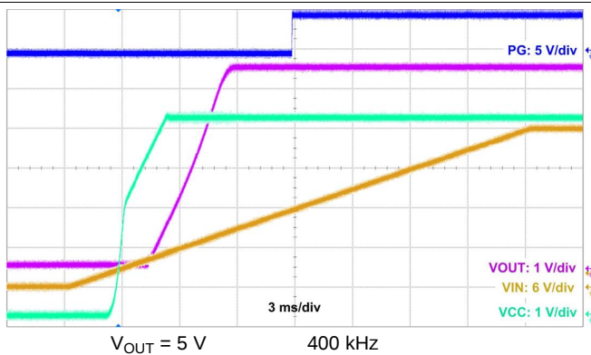
Figure 32. Start-Up Waveform
