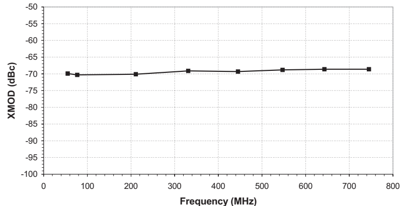
Figure 12: XMOD vs. Frequency (110 channels, +40 dBmV power, flat)
