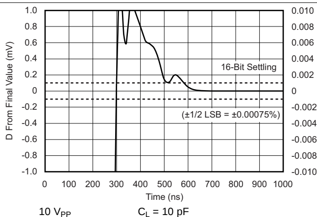
Figure 32. Large-Signal Positive Settling Time
