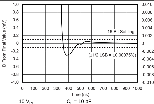
Figure 32. Large-Signal Positive Settling Time
