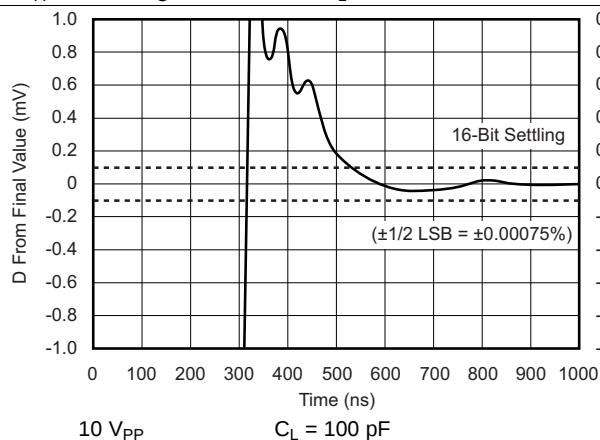
Figure 31. Large-Signal Positive Settling Time
