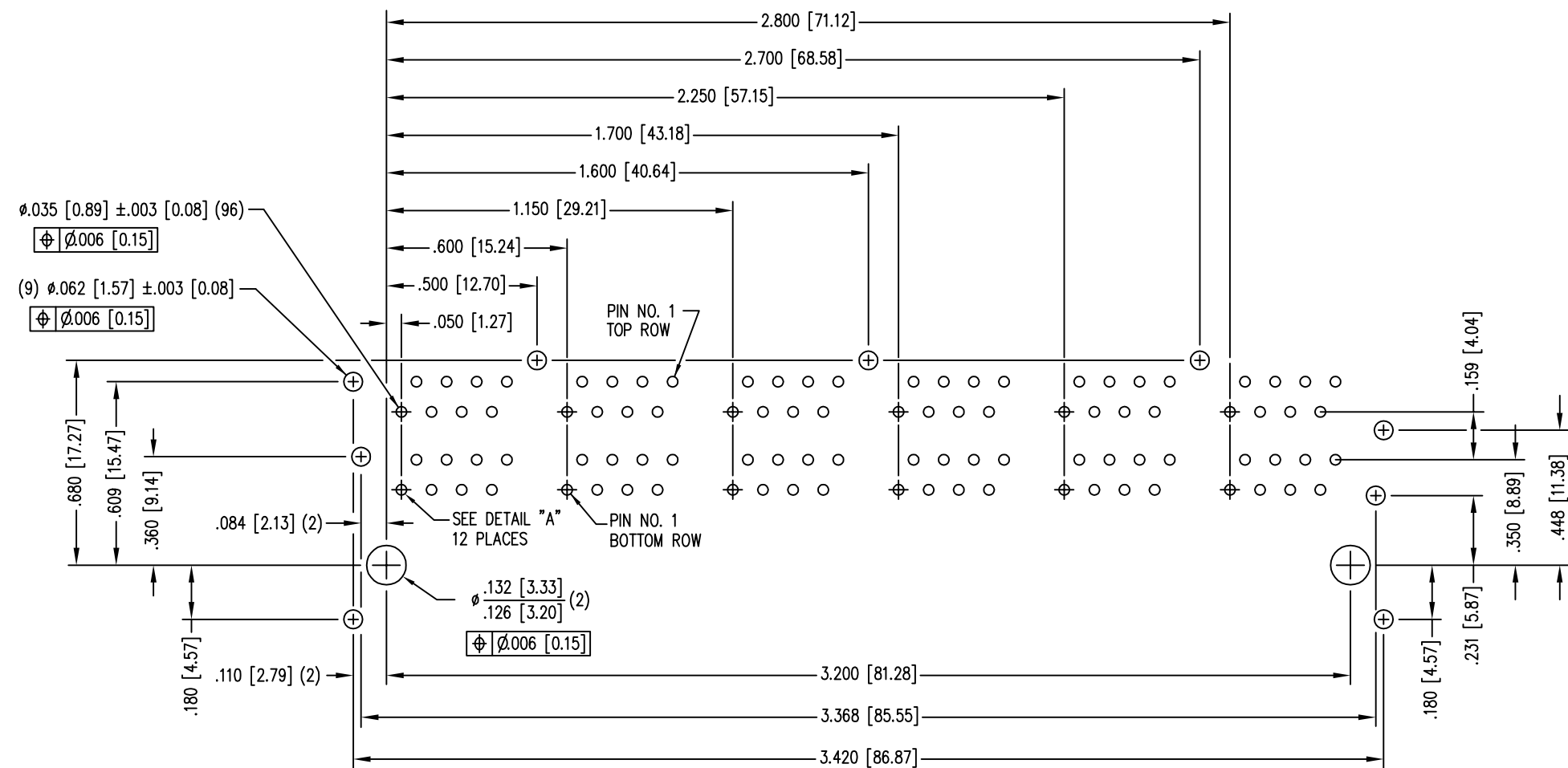
P.C.B. RECOMMENDED HOLE LAYOUT SEEN FROM COMPONENT SIDE ALL CENTERLINE DIMENSIONS ARE BASIC.
